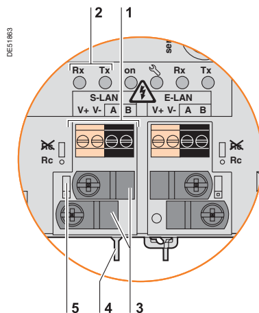
Порт S-LAN (ACE969TP)
